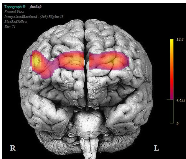
Figure 8. Projection of F-statistics map on brain surface image indicates right hemisphere dominance. Based on [x], BSpline interpolation was used to generate surface representation from F values of comparisons of manual vs. autonomous conditions along with thresholding determined by FDR.
